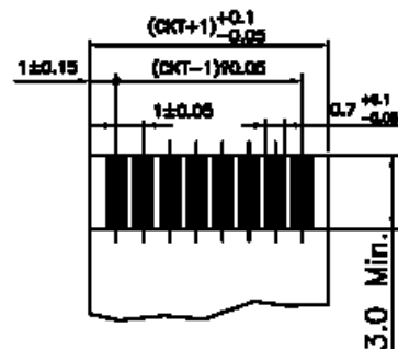
FPC/FPC DIMENSION THICKNESS 0.3 +0.05 / -0.03 mm
