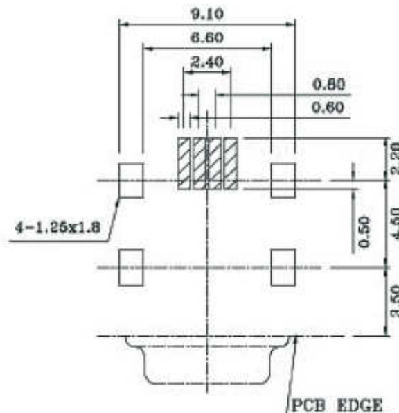
COMPONENT SIDE PCB LAYOUT
