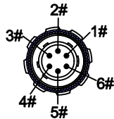
HR10A-7P-6P MALE
