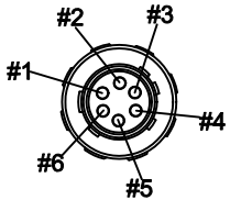
HR10A-7P-6S FEMALE
