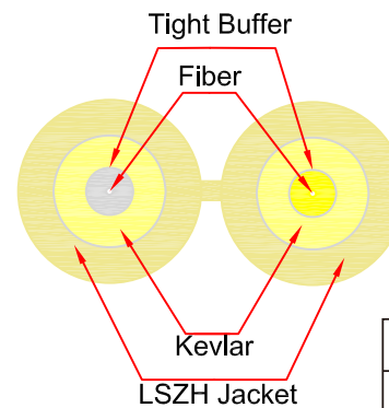
Cable Profile View
