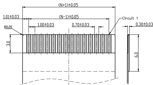
RECOMMENDED FPC/FFC DIMENSION
